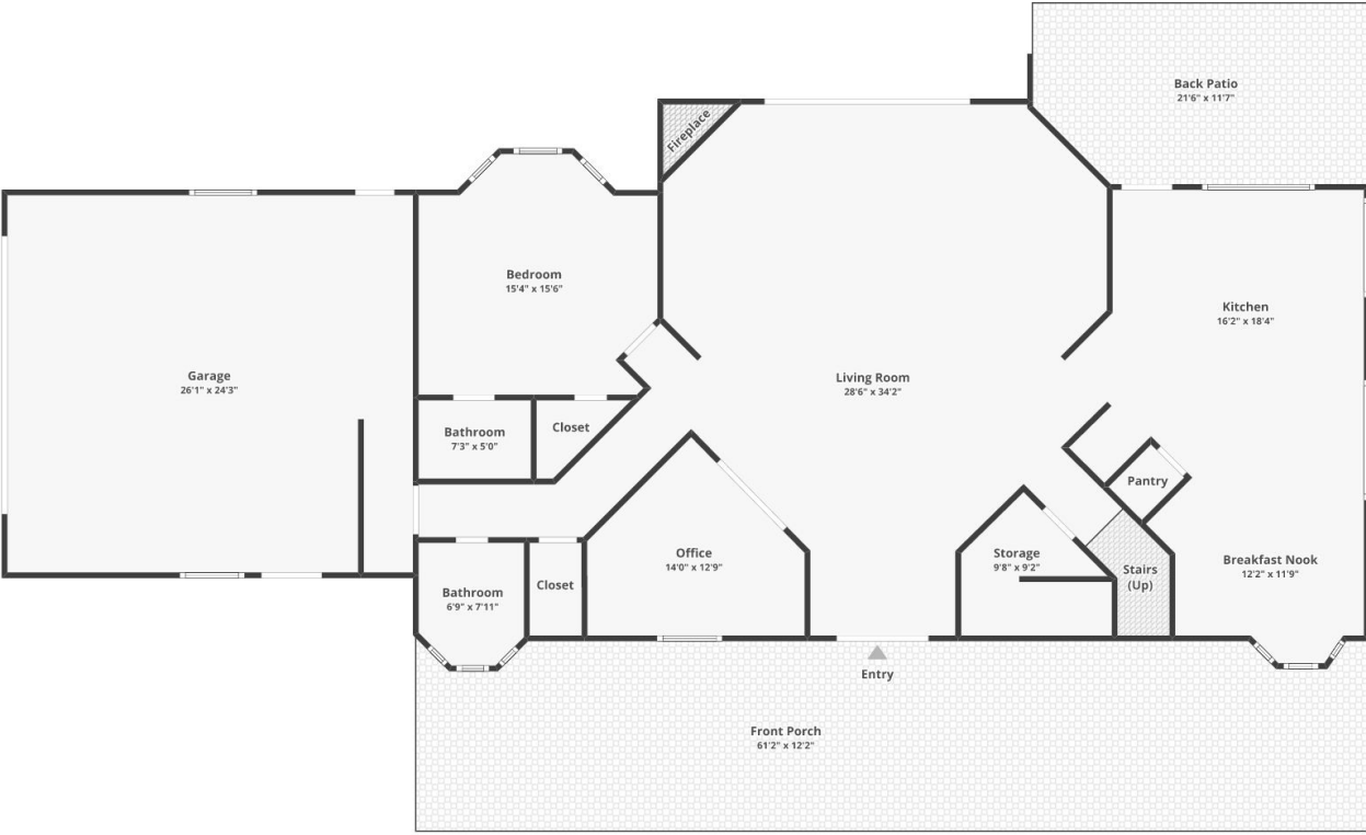
FLOOR 1
